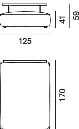
module seat L deep with back structure L110
