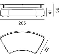
curved module seat M with back structure L205
