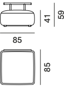
module seat S with back structure L70
