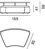
curved module seat S with back structure L155
