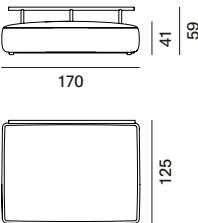
module seat L deep with back structure L155
