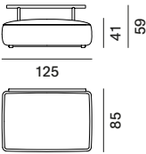
module seat M with back structure L110
