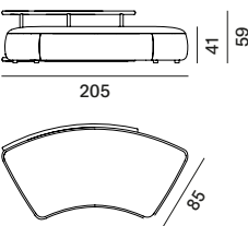
curved module seat M with back structure L155 L/R
