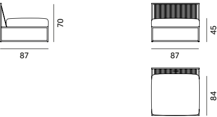
intermediate unit
